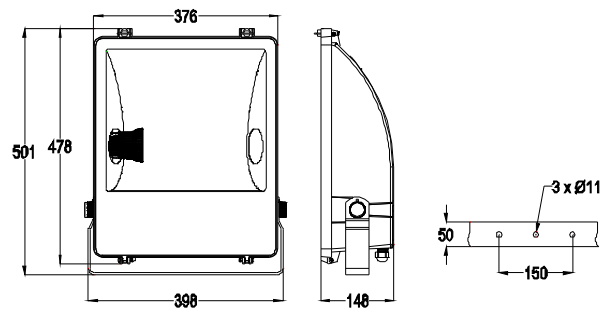
S2028 - Asy
