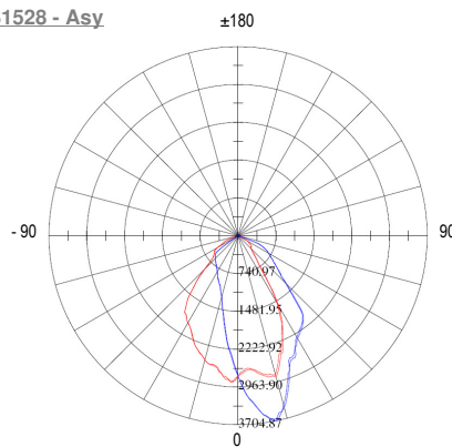
S1528 - Asy
