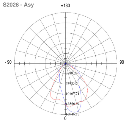
S2028 - Asy
